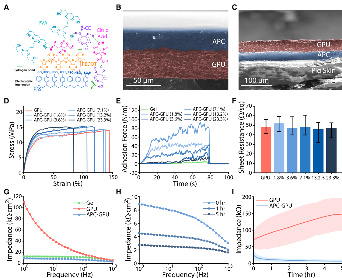
Figure 2. APC-GPU electrodes
